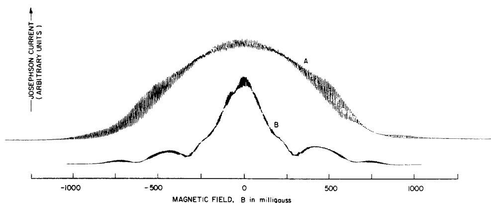
FIG. 2. Josephson current vs magnetic field for two junctions in parallel showing interference effects. Magnetic field applied normal to the area between junctions. Curve (A) shows interference maxima spaced at \Delta B = 8.7 \times 10^{-3} G, curve (B) spacing \Delta B = 4.8 \times 10^{-3} G. Maximum Josephson current indicated here is approximately 10^{-3} A.
